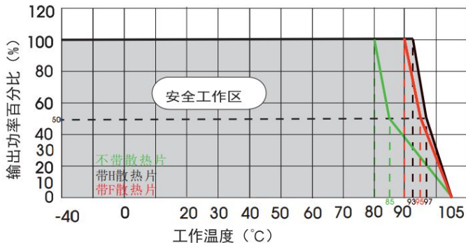
WLD10-H1D24/28/48/54(F/H)温度降额曲线 (Vin=110V, 无风)
