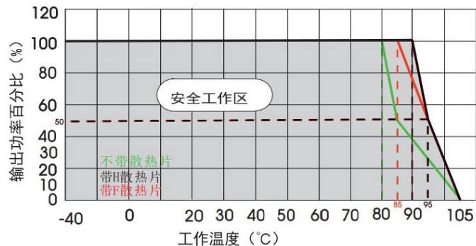
WLD10-H1D03/05/12/15(F/H)温度降额曲线 (Vin=110V, 无风)
