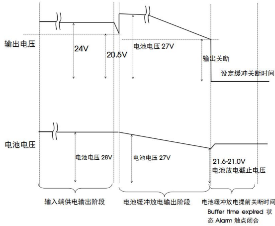
Buffer time expired 状态定义
