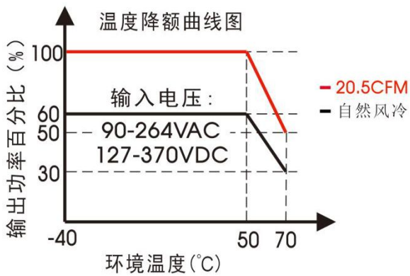
24/27/36/48/54V-C(满载 350W 带 20.5CFM 风扇)
