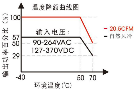
24/27/36/48/54V-C(满载 350W 带 20.5CFM 风扇)
